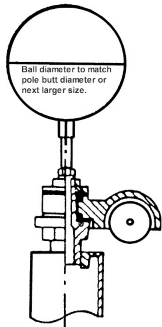
Truck Detail
